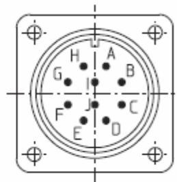
10 pin plug
