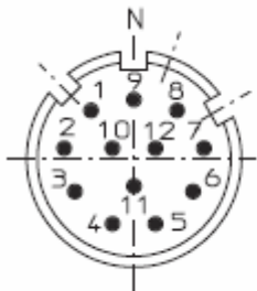
12 pin plug
