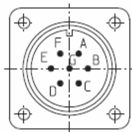
7 pin plug
