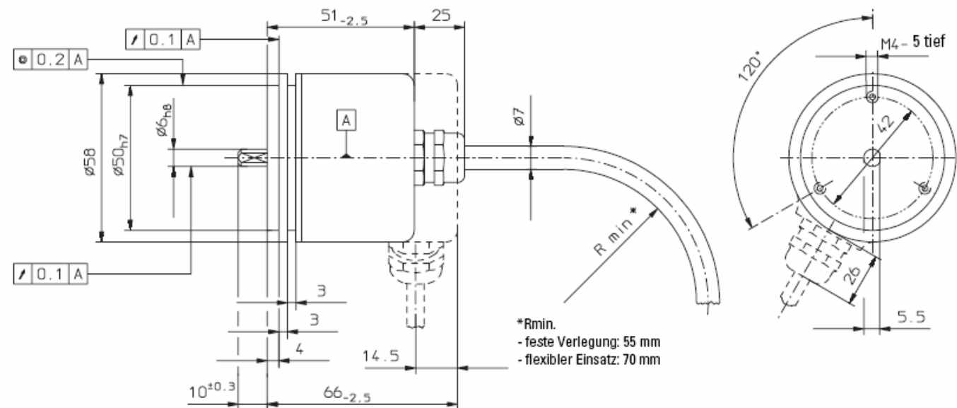
Synchroflansch \varnothing 58
