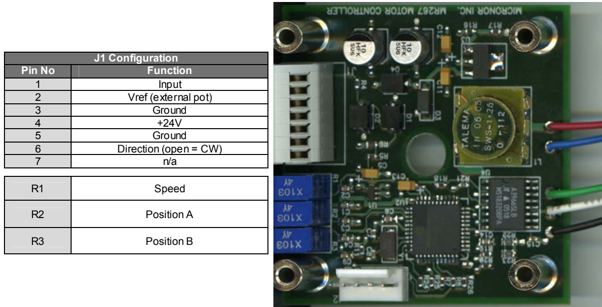
Figure 3. Wiring Reference For MR267 CLC Board.
